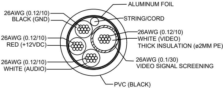
CABLE BUILDUP
