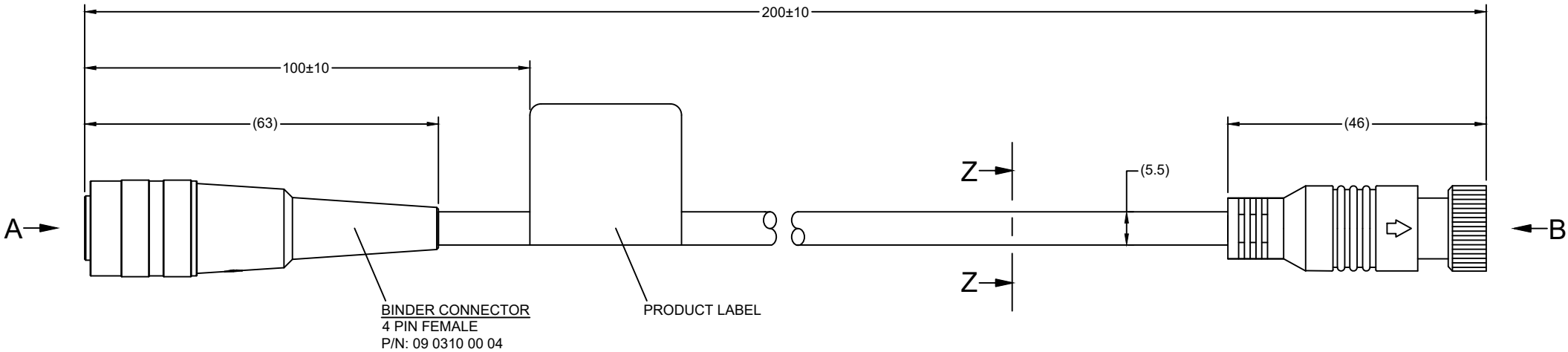
VIEW A
