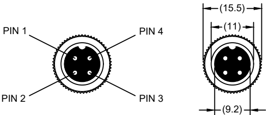
4 PIN FEMALE MATING FACE
