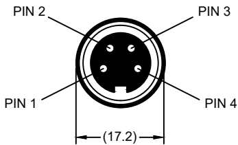
4 PIN FEMALE MATING FACE
